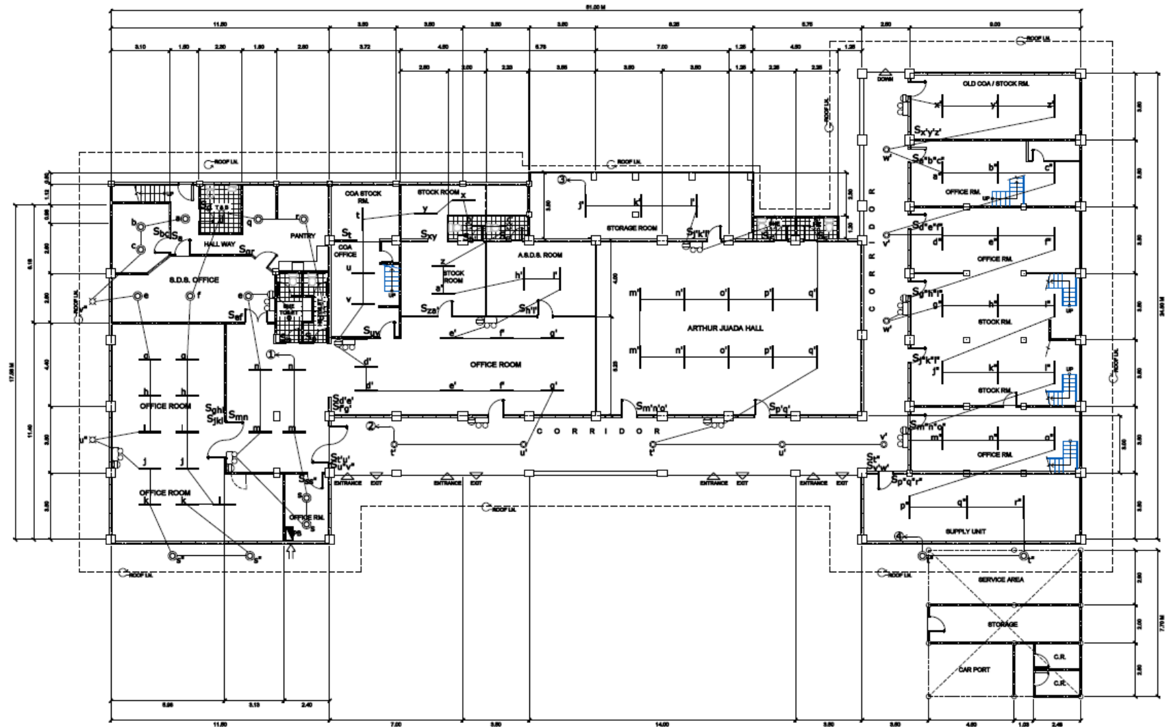
( OLD SCHOOL DIVISION OF ARLAN ) LIGHTING LAYOUT SCALE 1:100M
