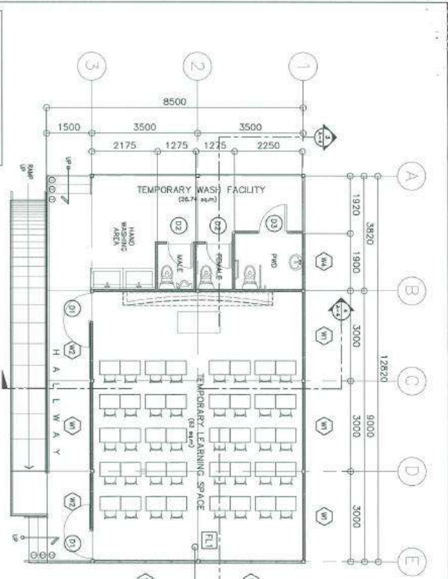
2 GROUND FLOOR PLAN SCALE 1:100 M
