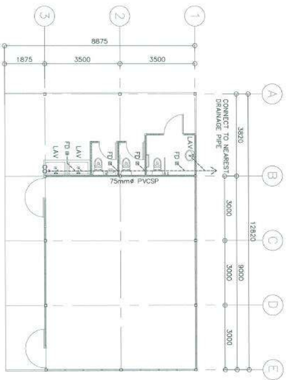
1 DRAINAGE LINE LAYOUT P-2 SCALE 1:100 M.
